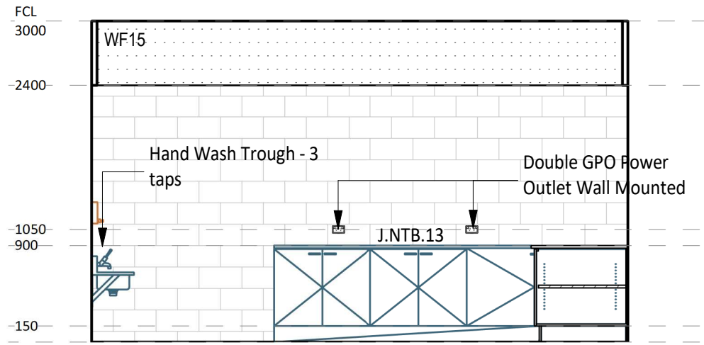
2 ELEVATION DETAIL 60-016 1 : 50
