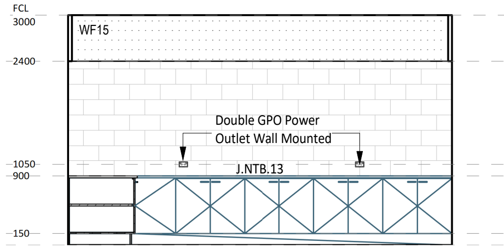
4 ELEVATION DETAIL 60-016 1 : 50
