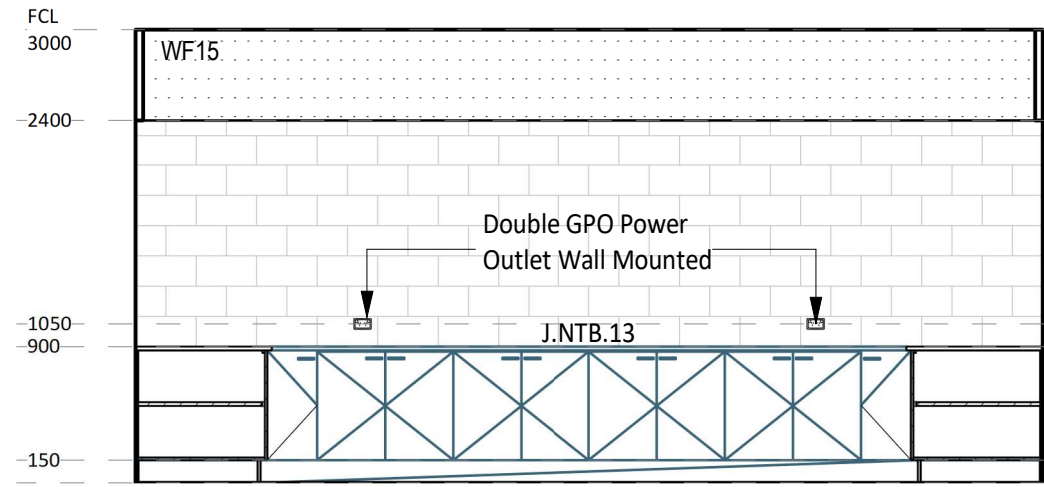
3 ELEVATION DETAIL 60-015 1 : 50
