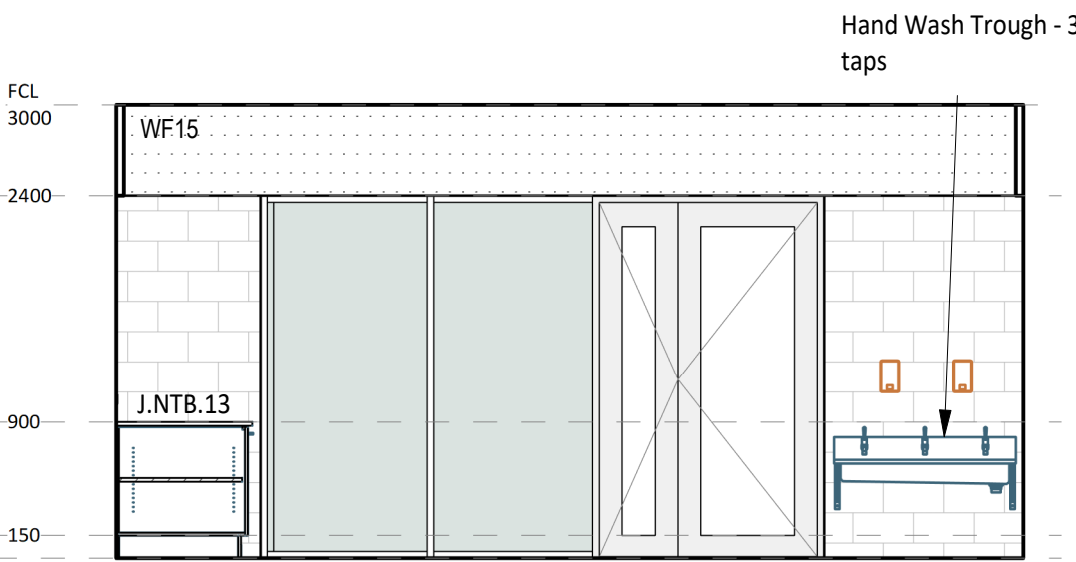
5 ELEVATION DETAIL 60-015 1 : 50
